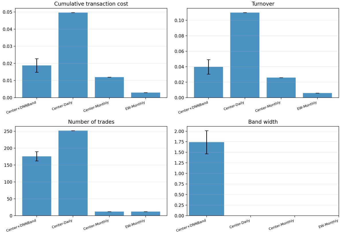
Figure 4: Stage 2 cost and turnover comparison across methods: cumulative transaction cost, turnover, trade count, and band width. Bars show the five-seed mean; error bars show the 95% training-seed interval. Band width bars are blank for methods without a band-width concept (structural, not zero).
